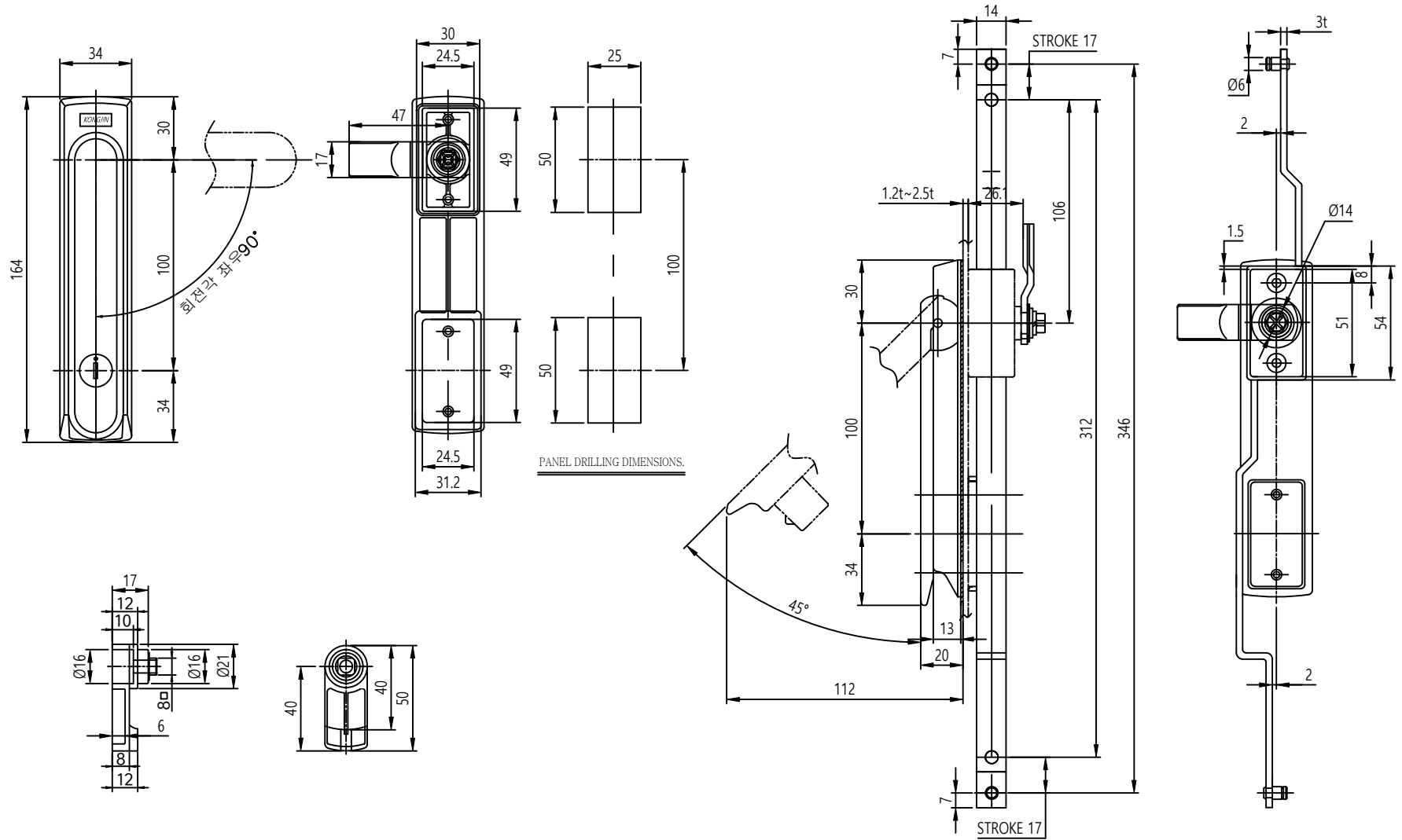
3 POINT LOCK HANDLE
